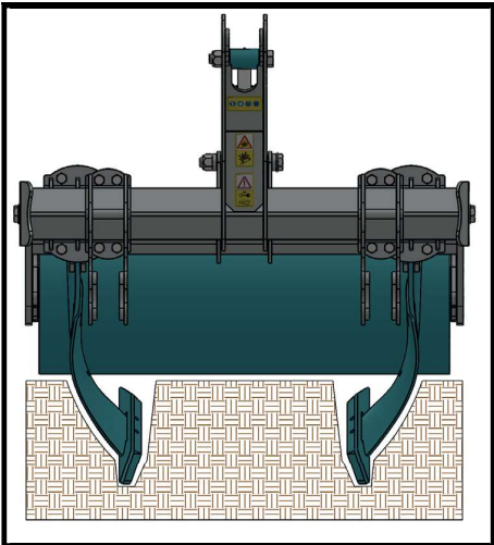
ANCHORS CURVED
